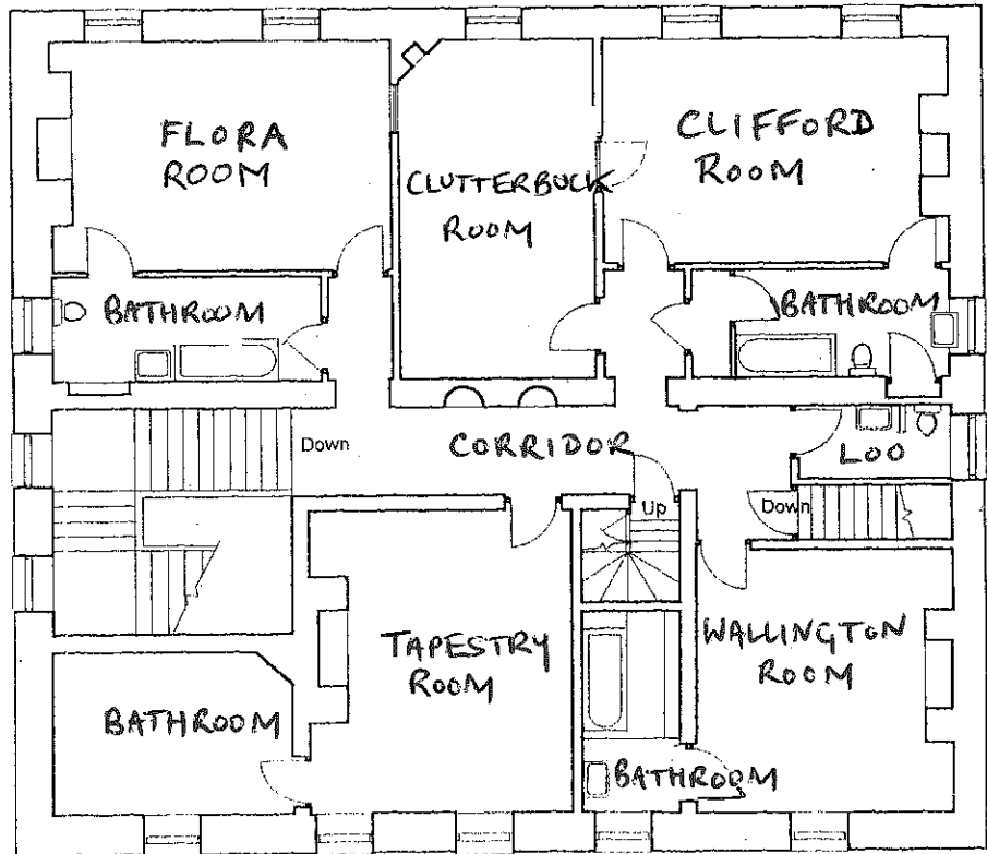
FIRST FLOOR
